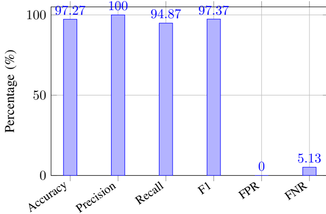
Fig. 3. AirSketch pinch-detection evaluation metrics.
